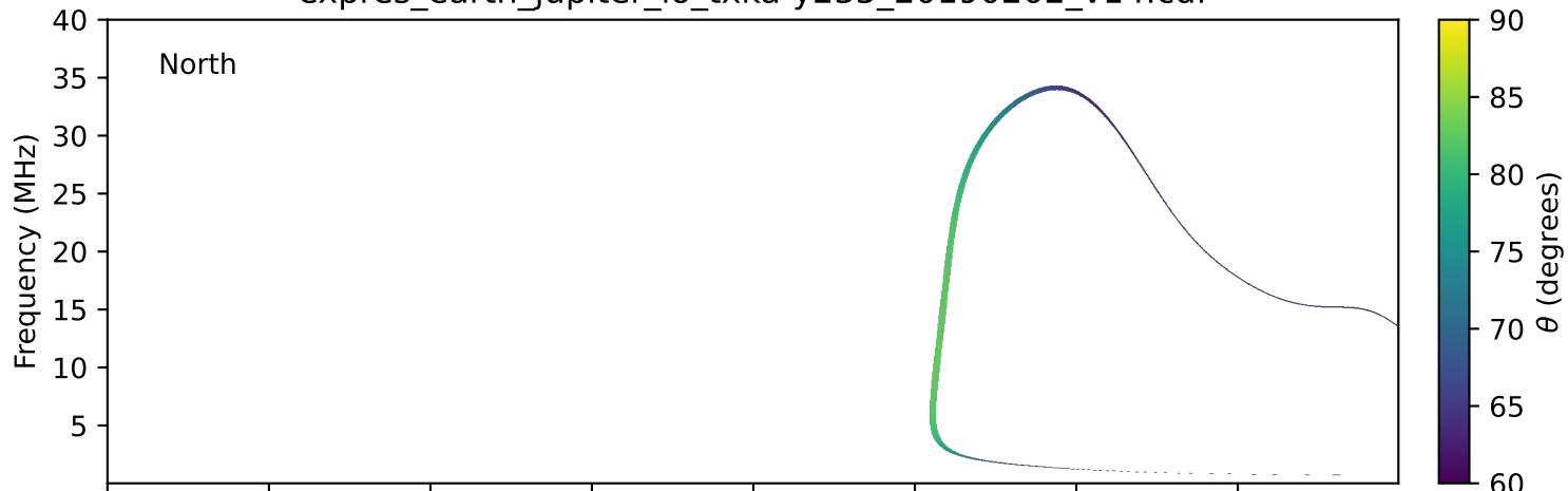
expres_earth_jupiter_io_txka-y235_20190202_v14.cdf
