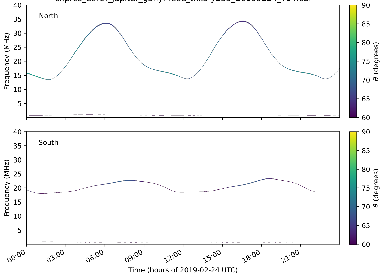
expres_earth_jupiter_ganymede_txka-y235_20190224_v14.cdf
