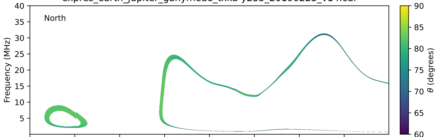
expres_earth_jupiter_ganymede_txka-y235_20190223_v14.cdf
