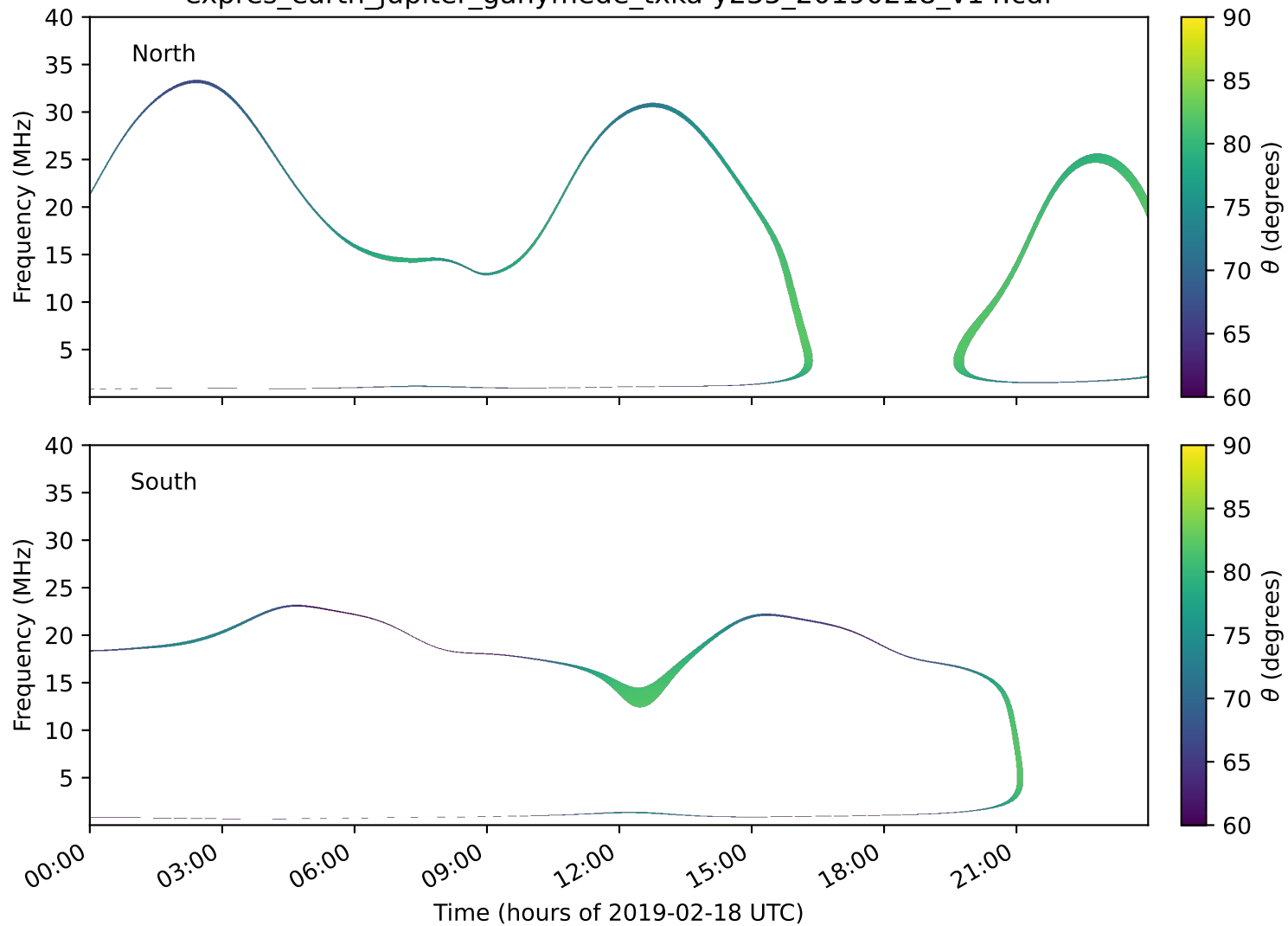
expres_earth_jupiter_ganymede_txka-y235_20190218_v14.cdf
