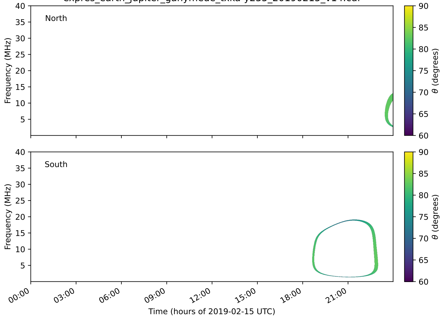
expres_earth_jupiter_ganymede_txka-y235_20190215_v14.cdf
