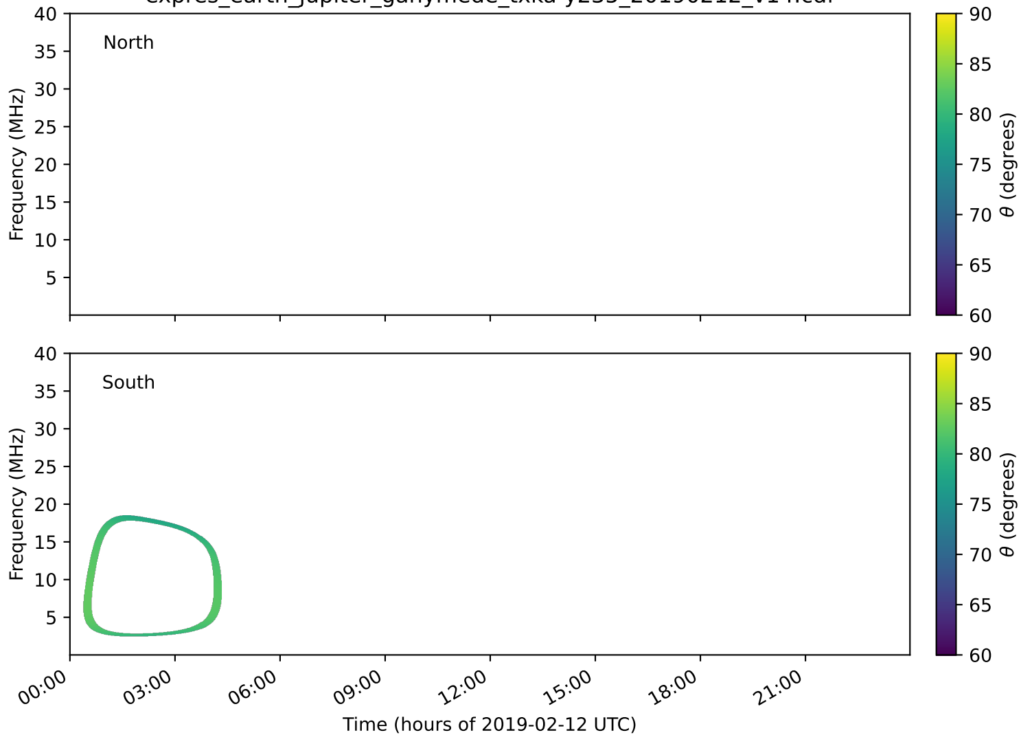
expres_earth_jupiter_ganymede_txka-y235_20190212_v14.cdf
