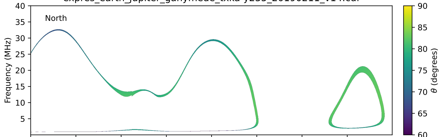
expres_earth_jupiter_ganymede_txka-y235_20190211_v14.cdf
