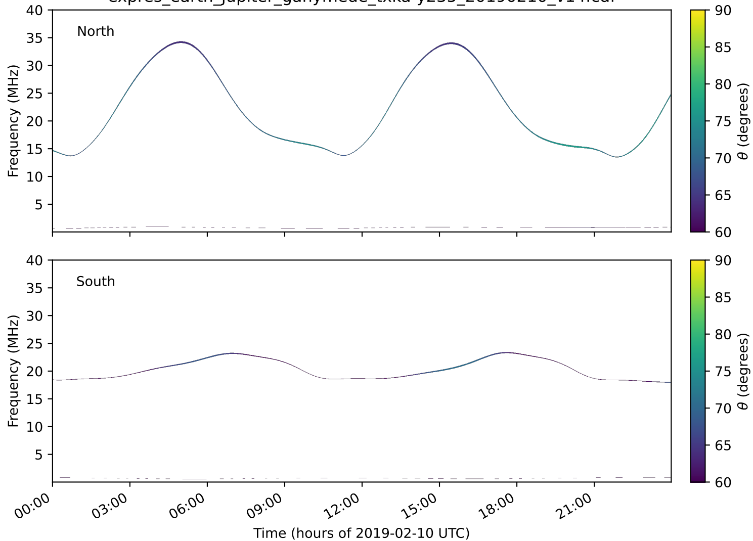
expres_earth_jupiter_ganymede_txka-y235_20190210_v14.cdf
