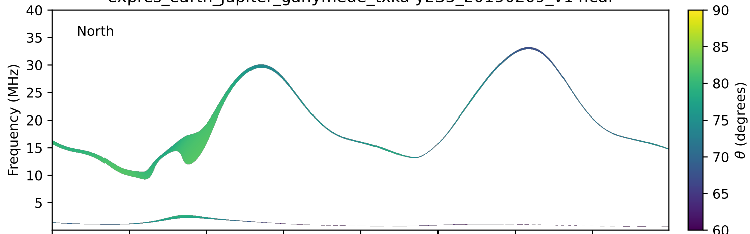
expres_earth_jupiter_ganymede_txka-y235_20190209_v14.cdf
