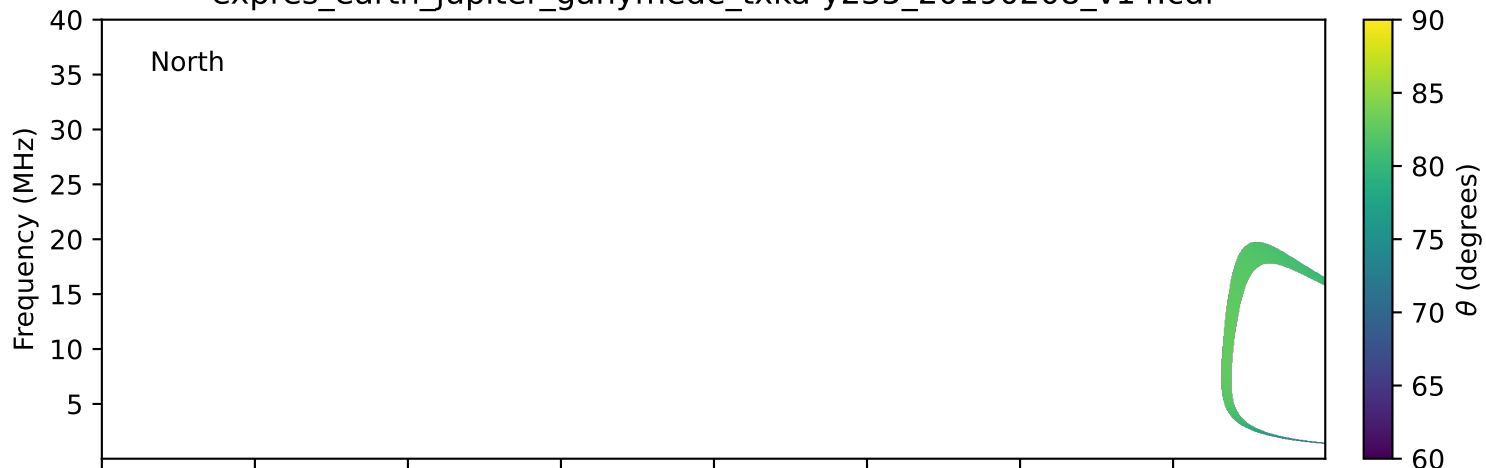
expres_earth_jupiter_ganymede_txka-y235_20190208_v14.cdf
