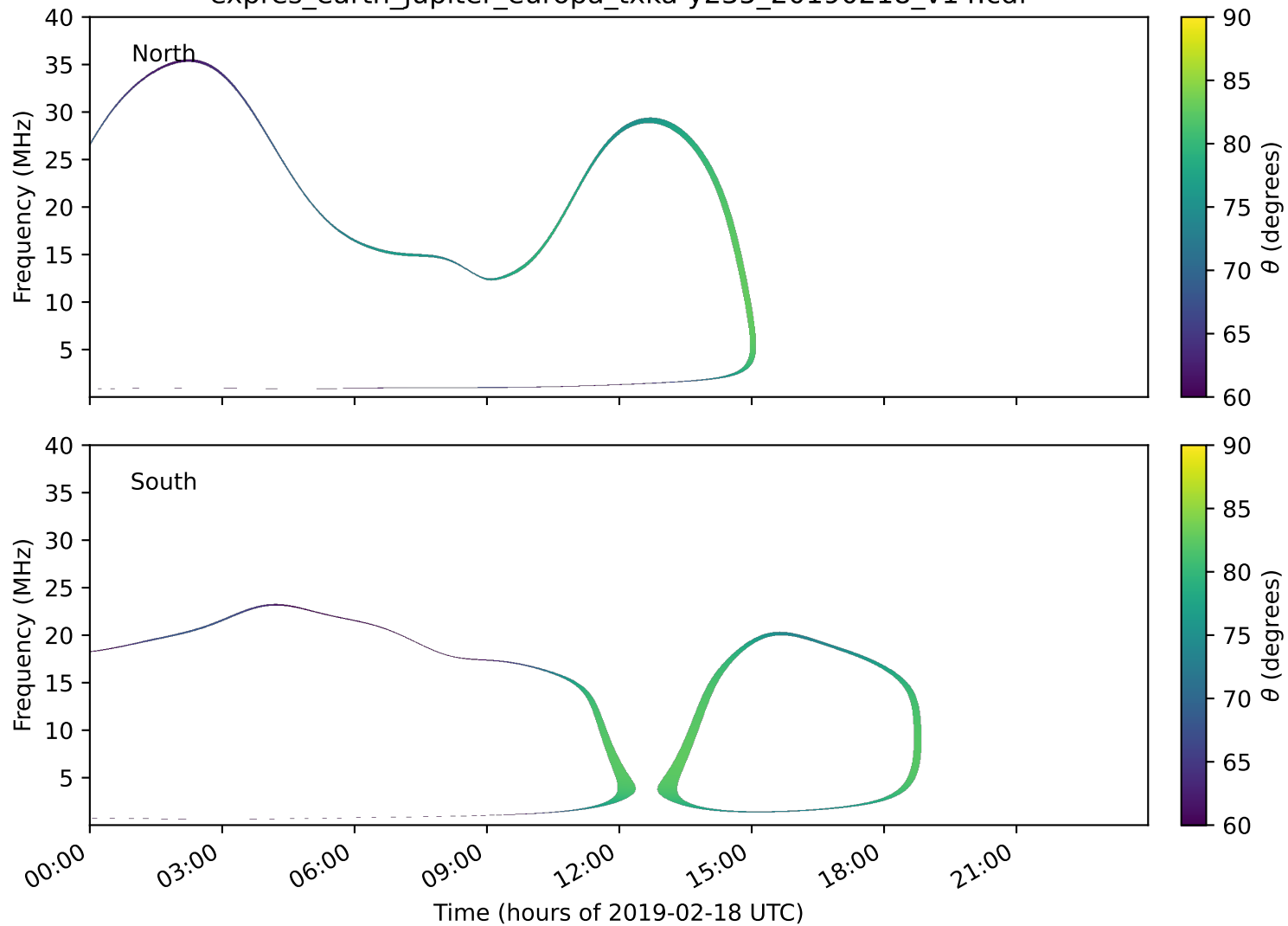
expres_earth_jupiter_europa_txka-y235_20190218_v14.cdf
