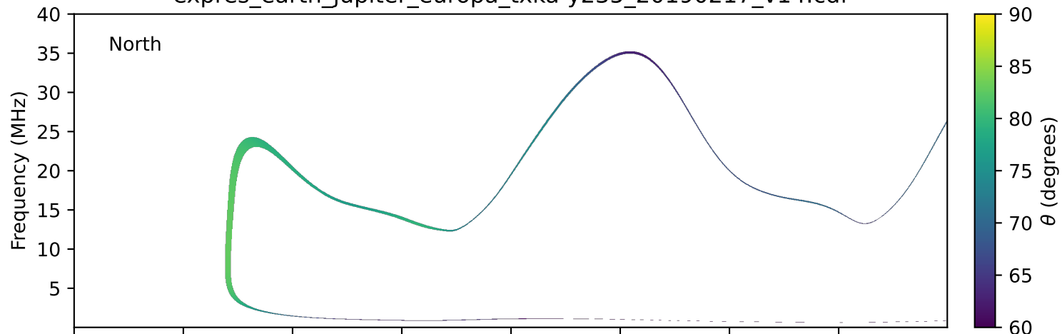
expres_earth_jupiter_europa_txka-y235_20190217_v14.cdf
