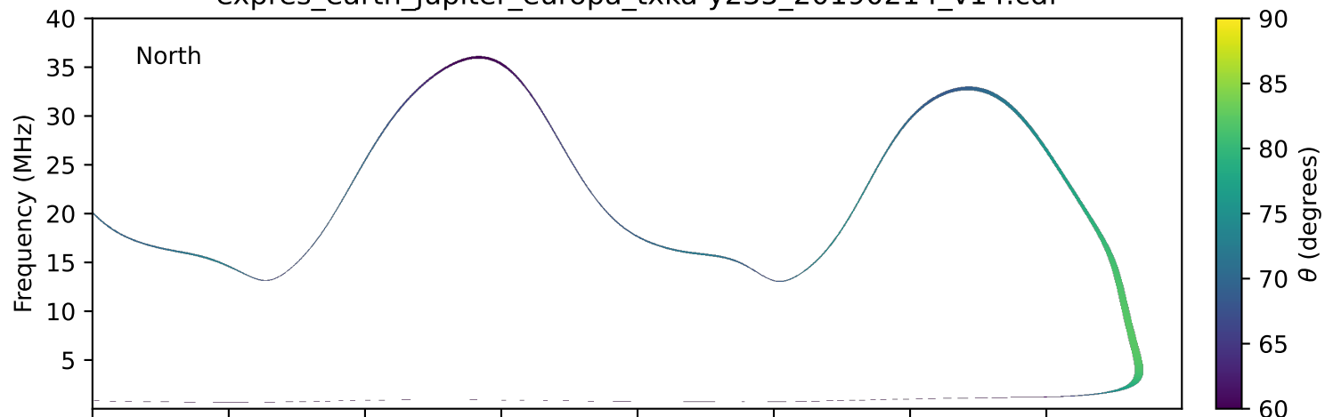
expres_earth_jupiter_europa_txka-y235_20190214_v14.cdf
