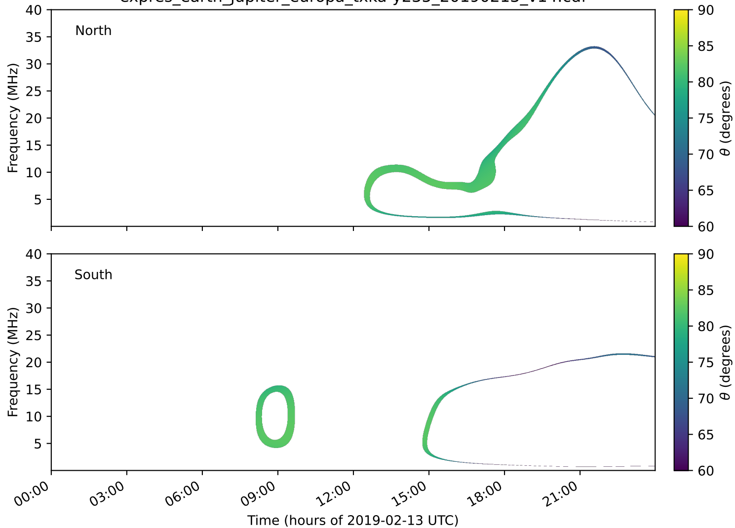
expres_earth_jupiter_europa_txka-y235_20190213_v14.cdf
