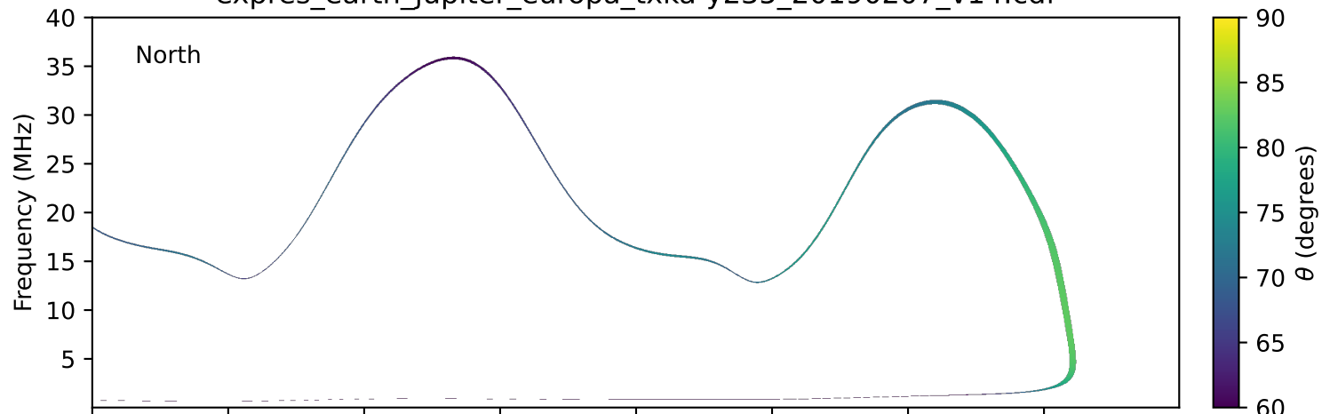
expres_earth_jupiter_europa_txka-y235_20190207_v14.cdf
