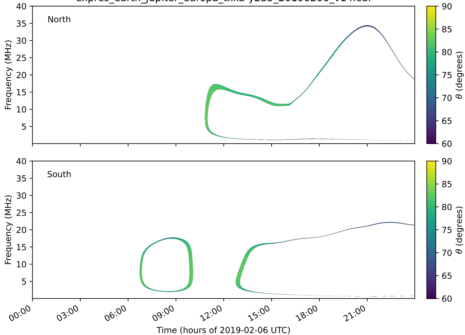
expres_earth_jupiter_europa_txka-y235_20190206_v14.cdf
