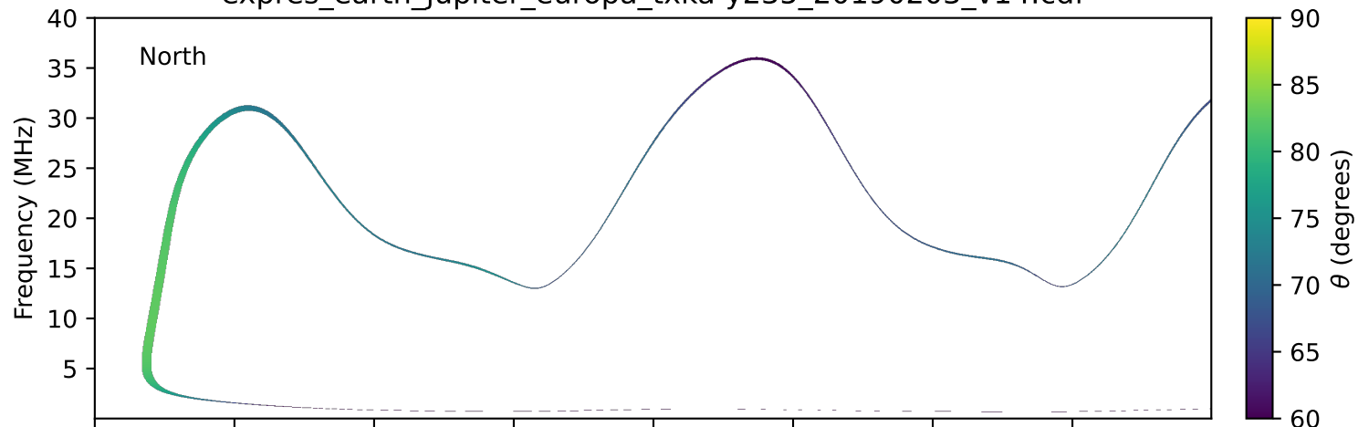
expres_earth_jupiter_europa_txka-y235_20190203_v14.cdf
