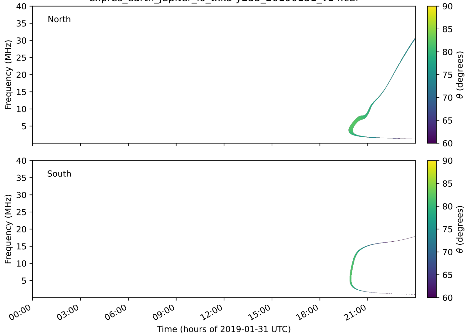
expres_earth_jupiter_io_txka-y235_20190131_v14.cdf
