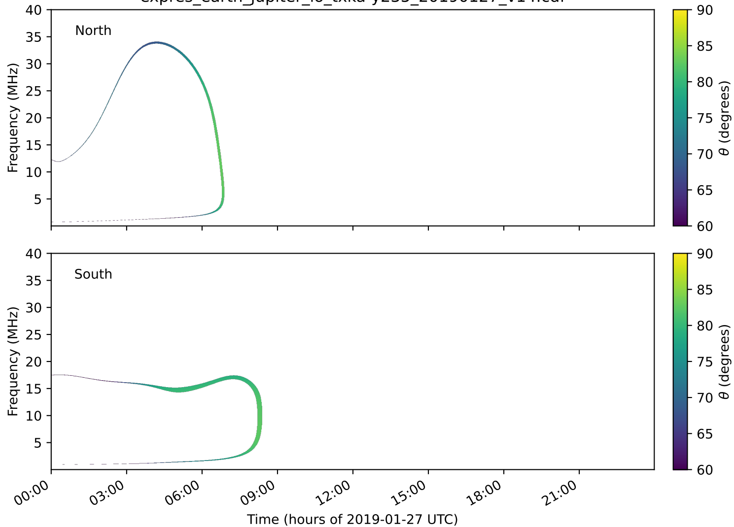
expres_earth_jupiter_io_txka-y235_20190127_v14.cdf
