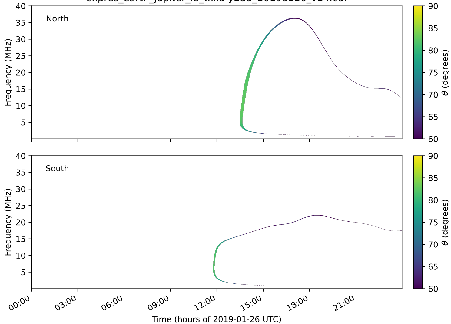
expres_earth_jupiter_io_txka-y235_20190126_v14.cdf
