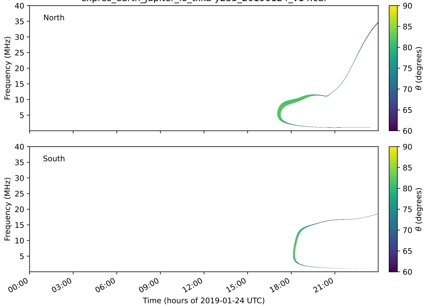
expres_earth_jupiter_io_txka-y235_20190124_v14.cdf
