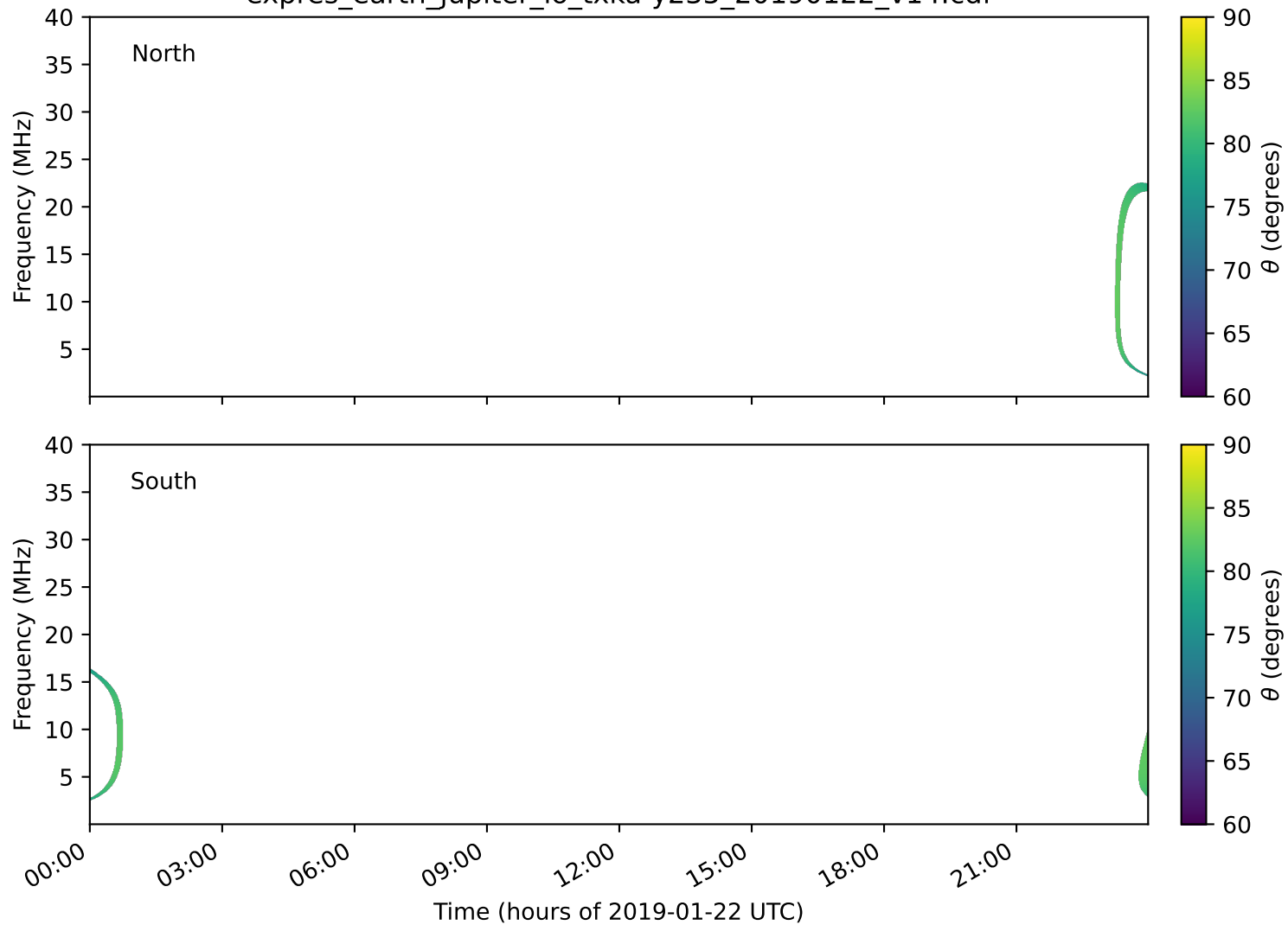
expres_earth_jupiter_io_txka-y235_20190122_v14.cdf
