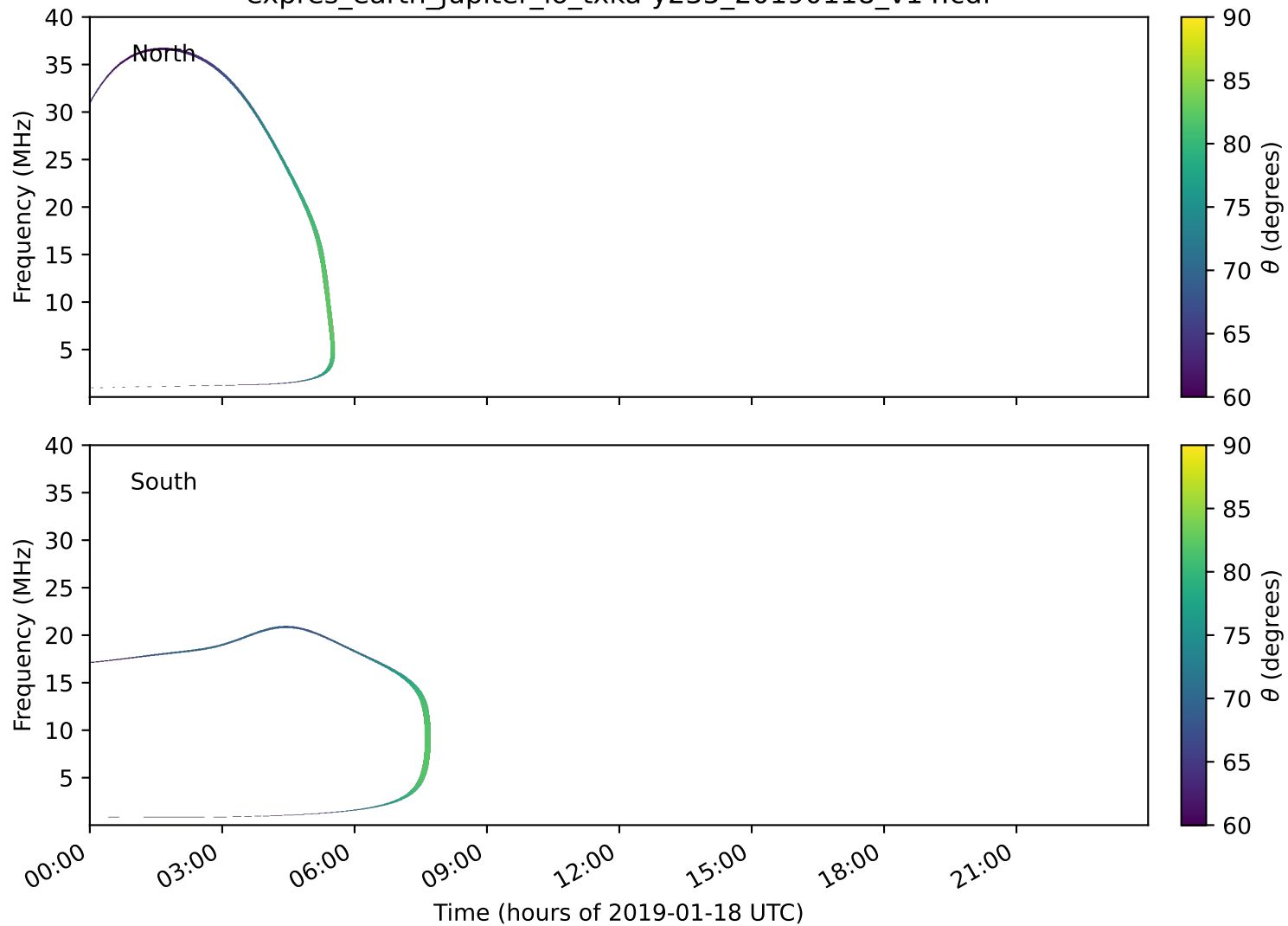
expres_earth_jupiter_io_txka-y235_20190118_v14.cdf
