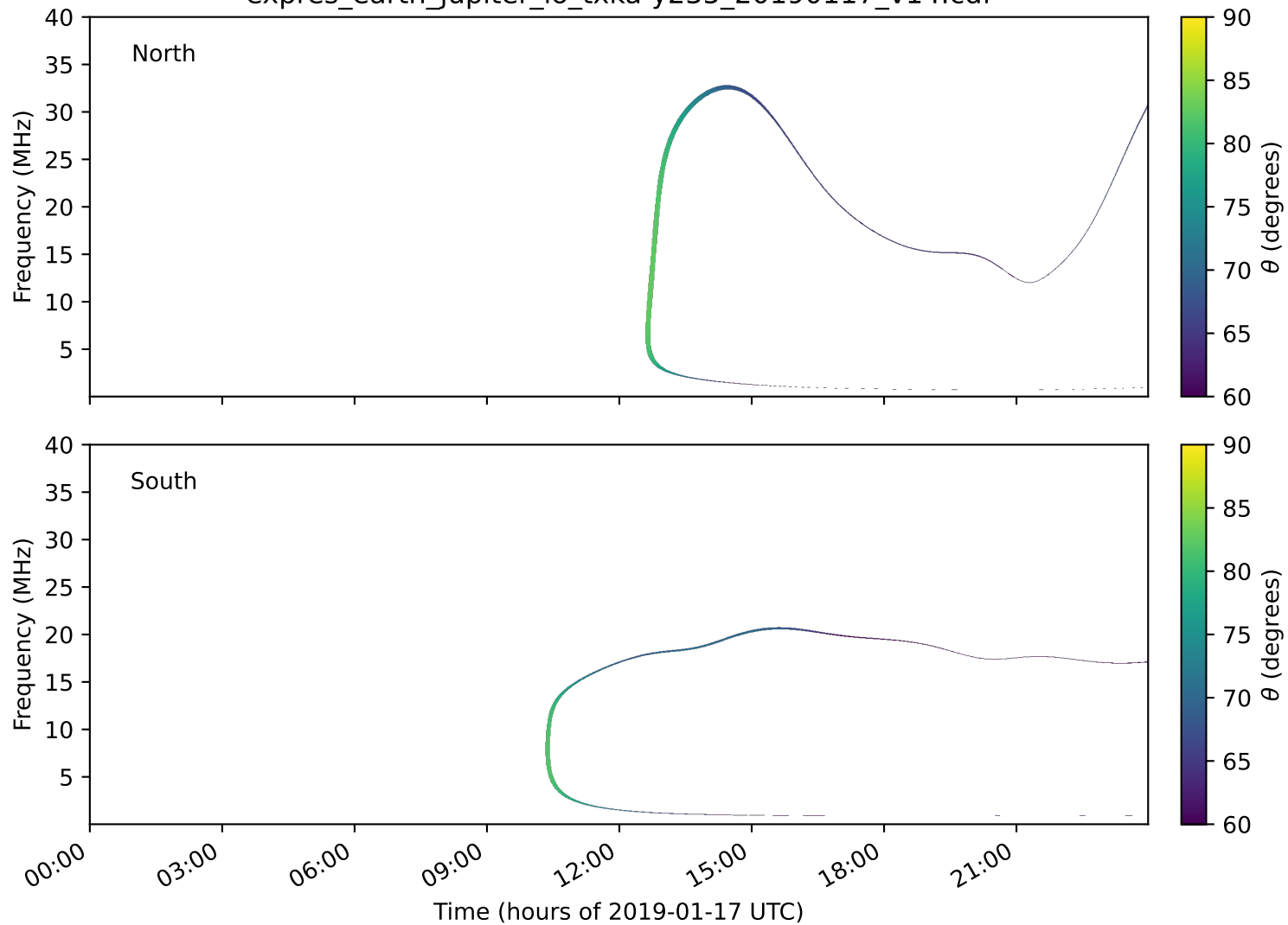
expres_earth_jupiter_io_txka-y235_20190117_v14.cdf
