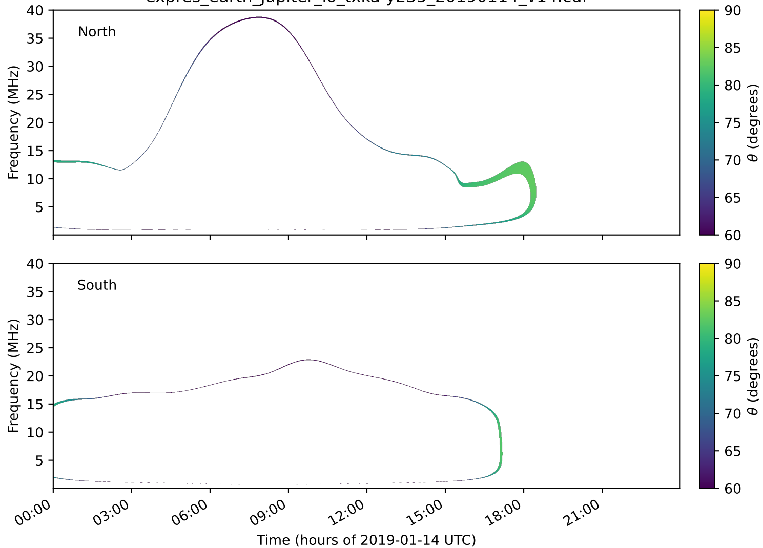
expres_earth_jupiter_io_txka-y235_20190114_v14.cdf
