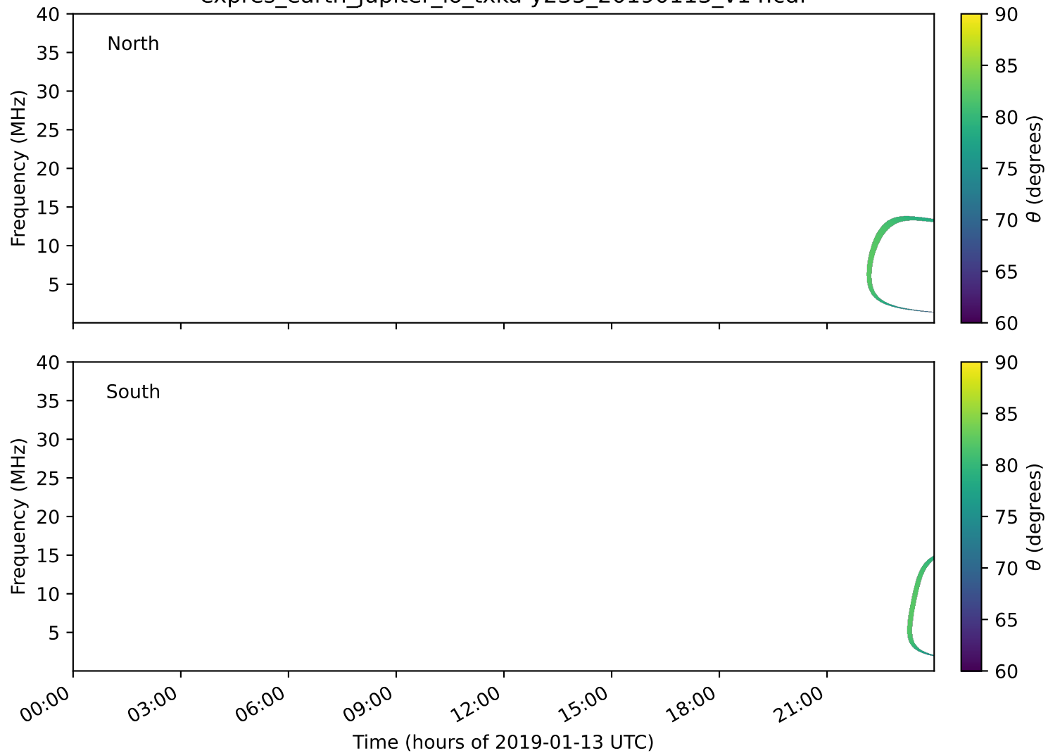
expres_earth_jupiter_io_txka-y235_20190113_v14.cdf
