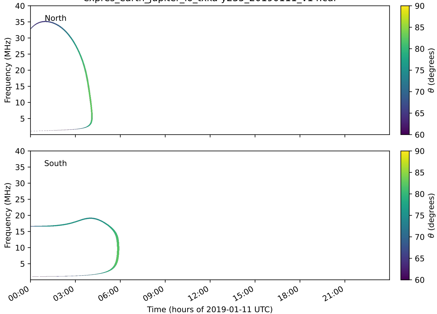
expres_earth_jupiter_io_txka-y235_20190111_v14.cdf
