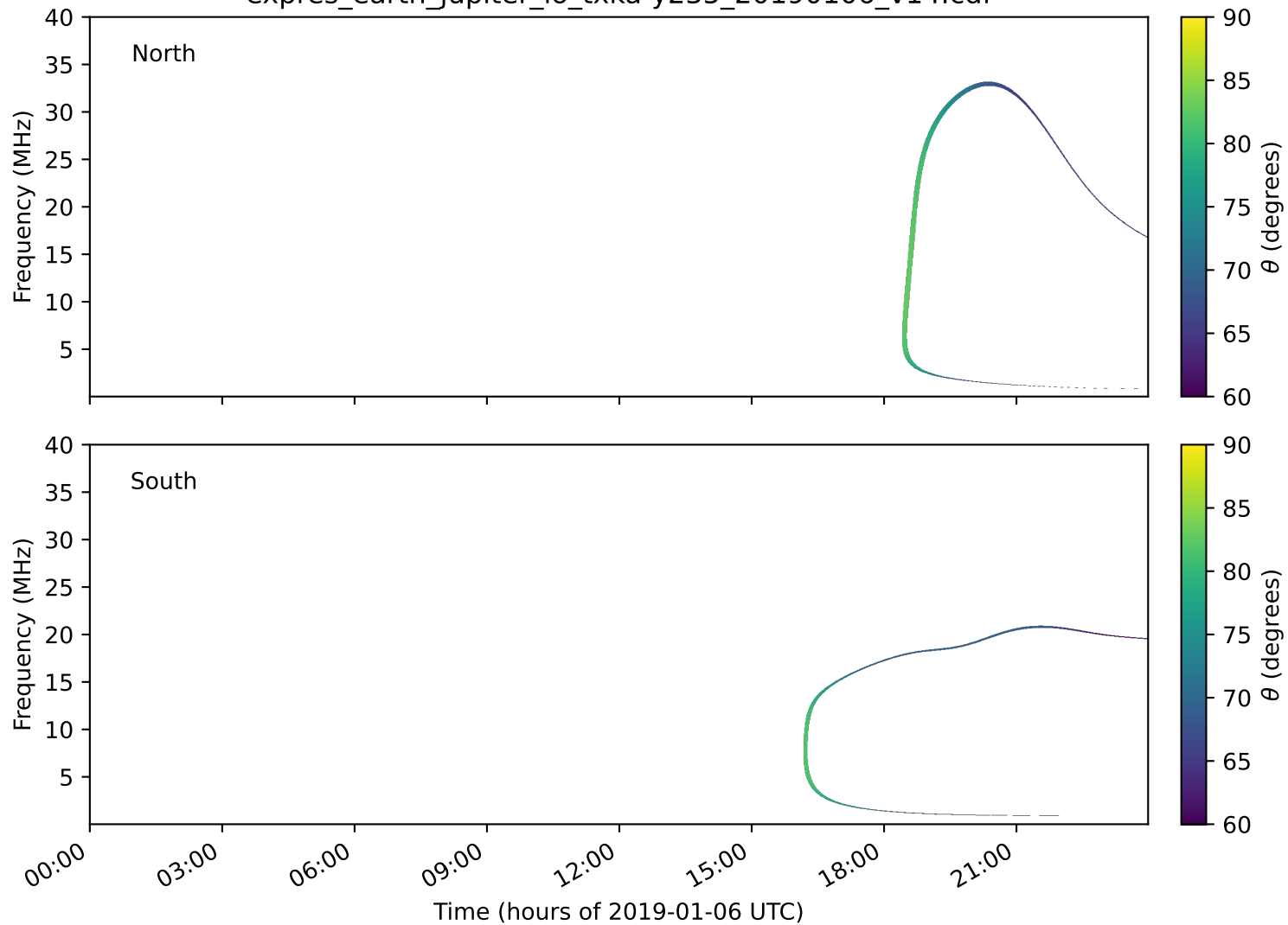
expres_earth_jupiter_io_txka-y235_20190106_v14.cdf
