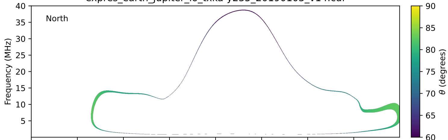
expres_earth_jupiter_io_txka-y235_20190103_v14.cdf
