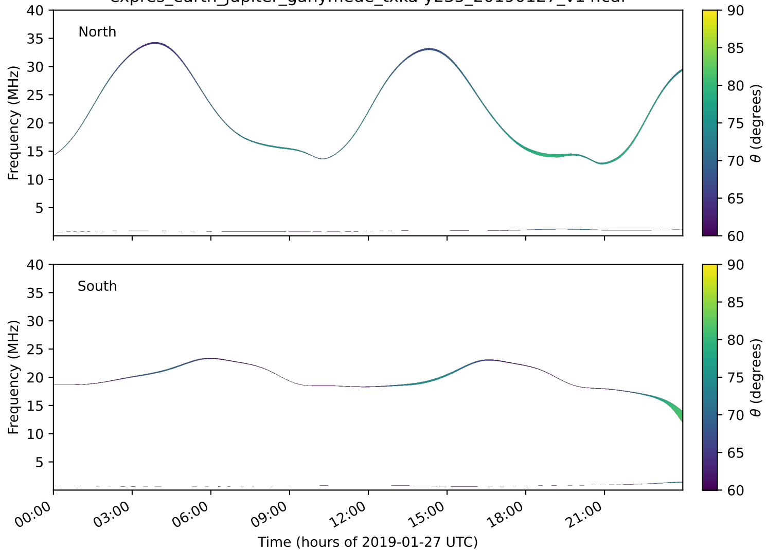
expres_earth_jupiter_ganymede_txka-y235_20190127_v14.cdf
