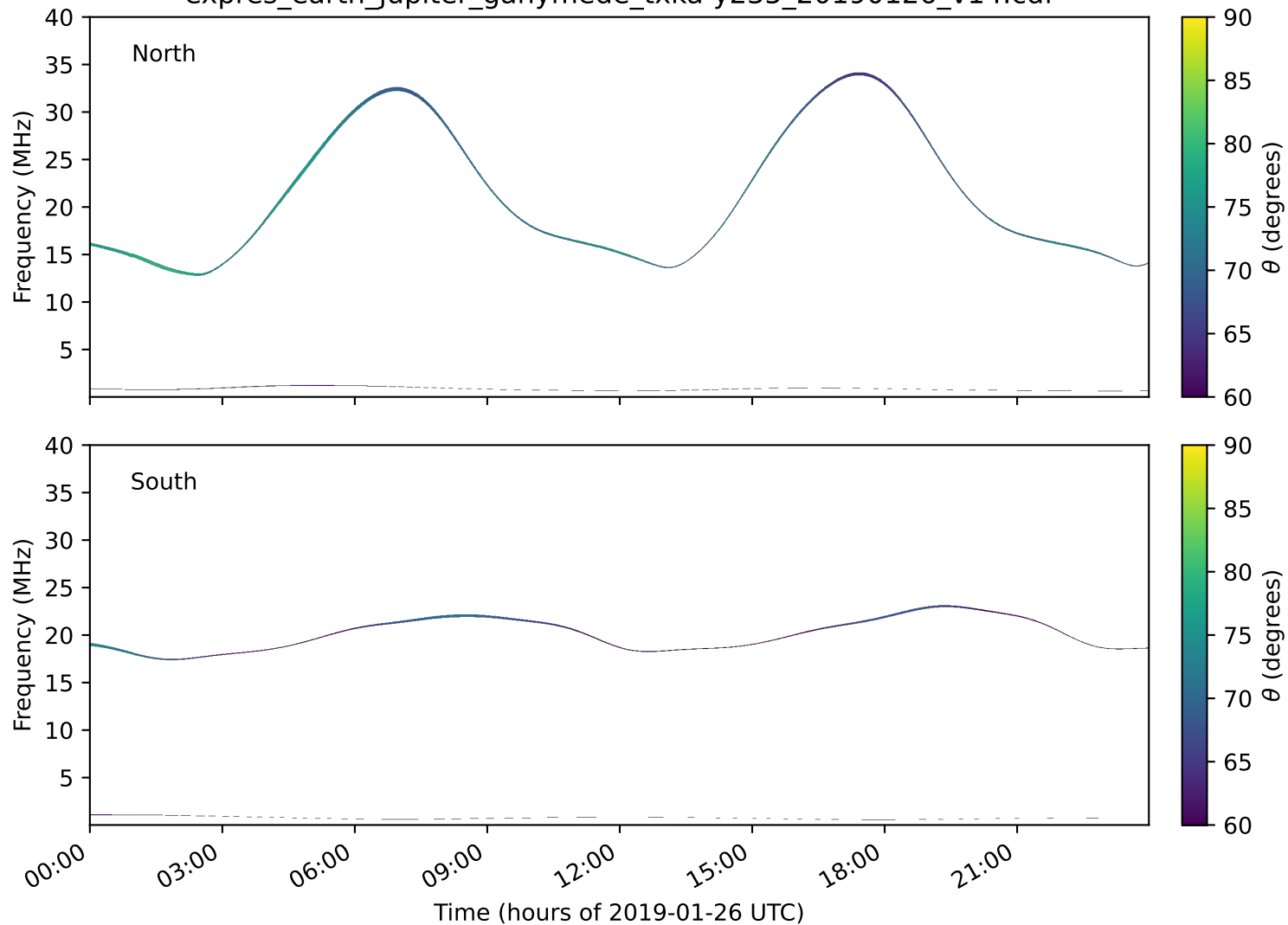
expres_earth_jupiter_ganymede_txka-y235_20190126_v14.cdf
