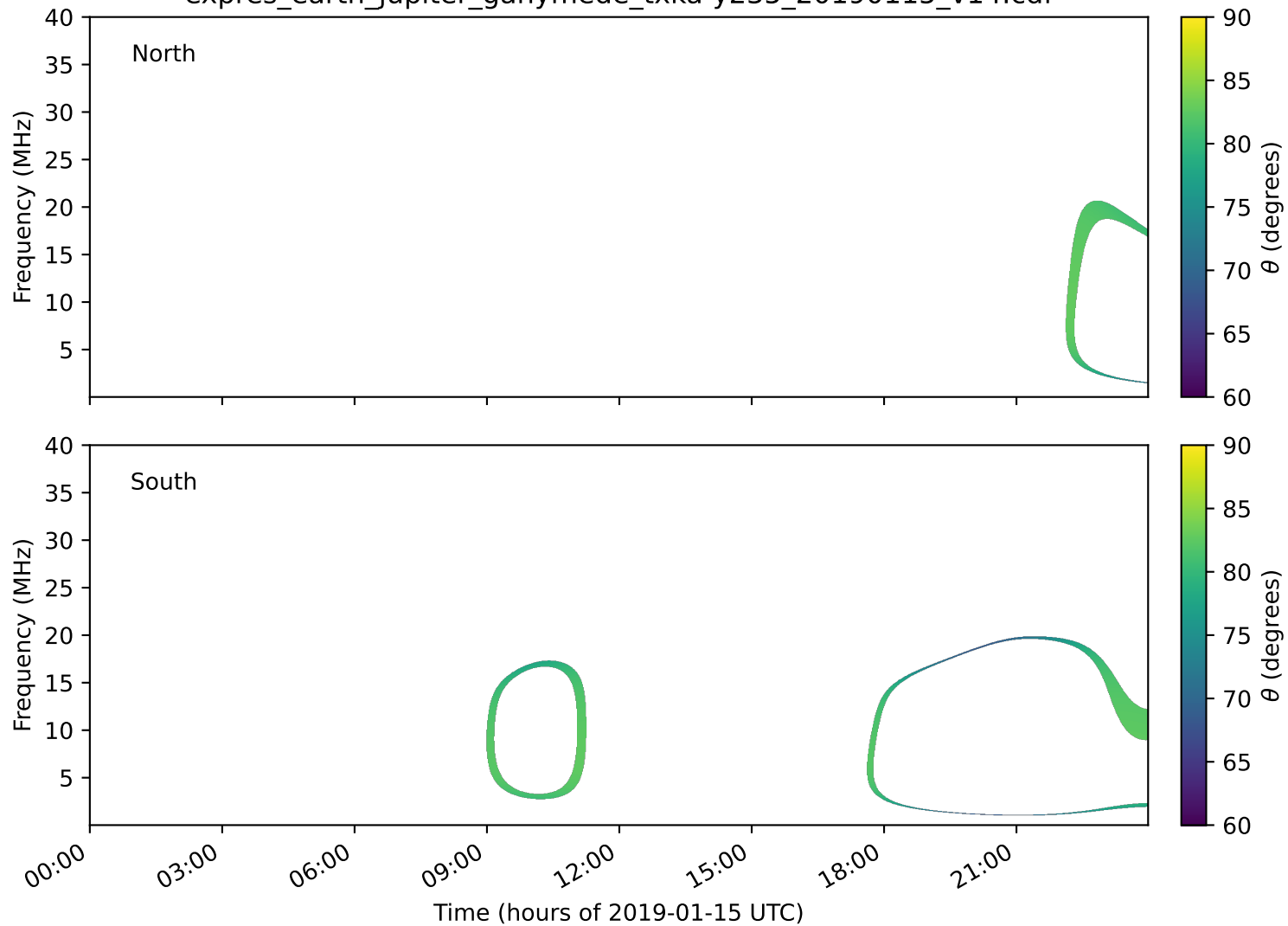
expres_earth_jupiter_ganymede_txka-y235_20190115_v14.cdf
