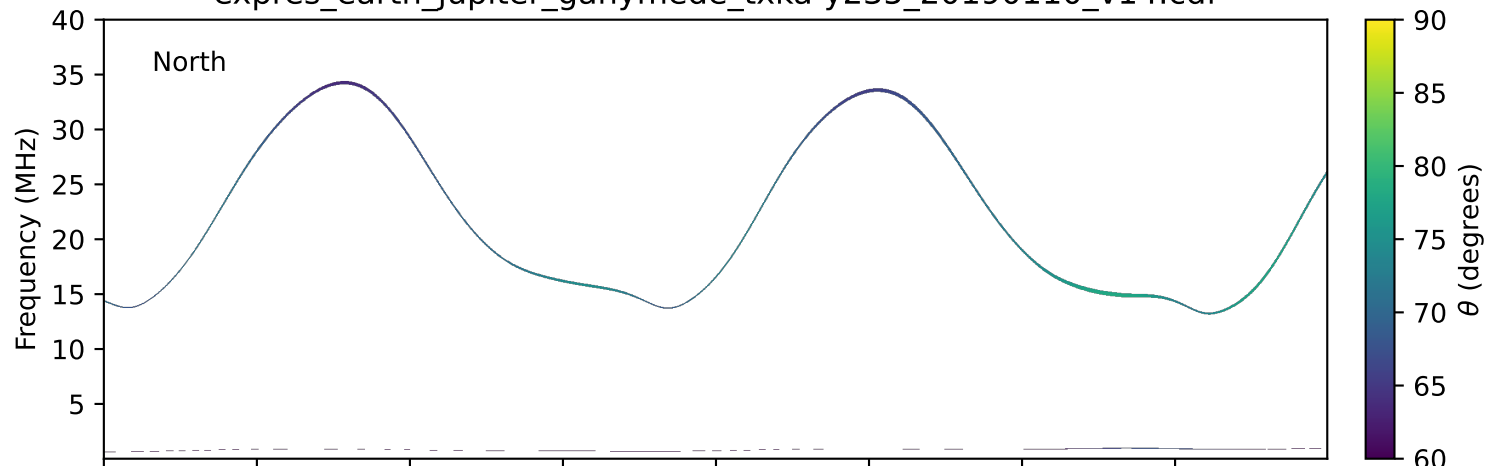
expres_earth_jupiter_ganymede_txka-y235_20190110_v14.cdf
