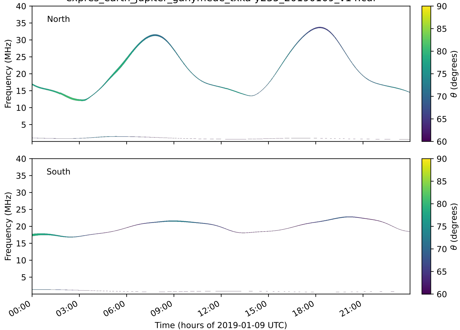
expres_earth_jupiter_ganymede_txka-y235_20190109_v14.cdf
