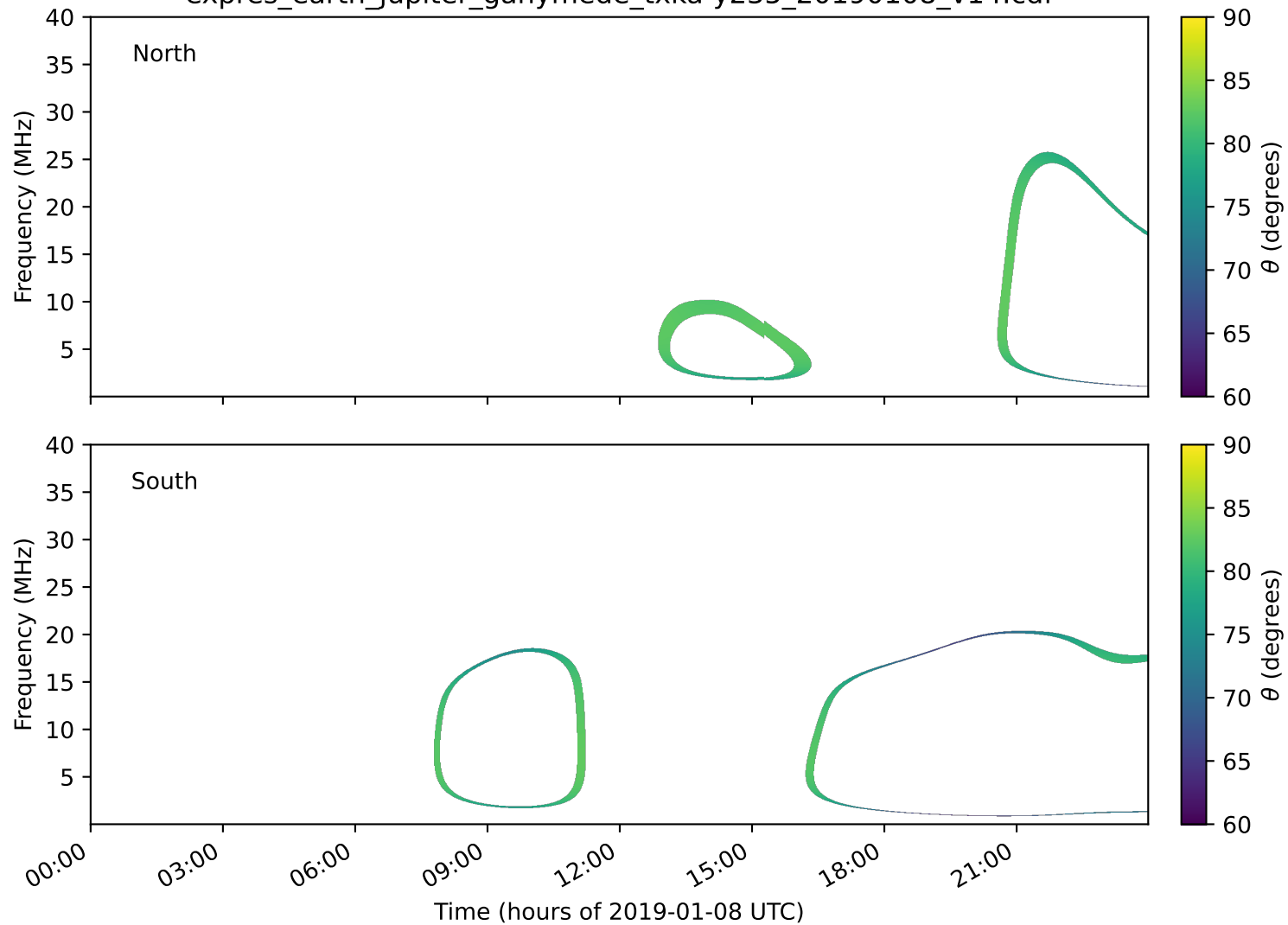
expres_earth_jupiter_ganymede_txka-y235_20190108_v14.cdf
