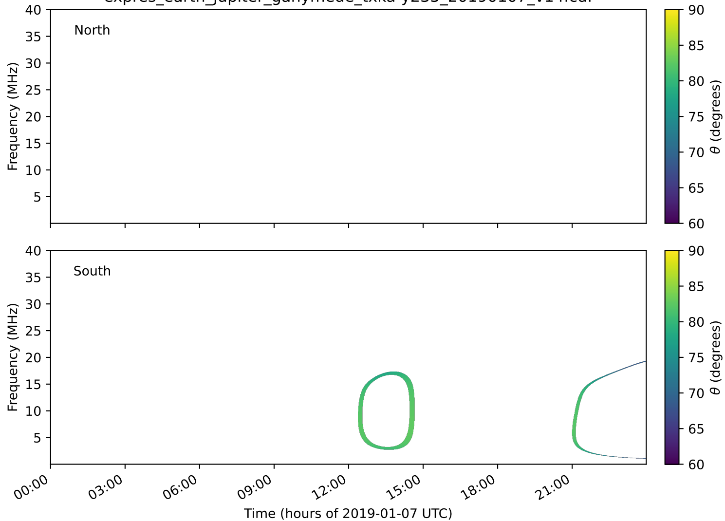
expres_earth_jupiter_ganymede_txka-y235_20190107_v14.cdf
