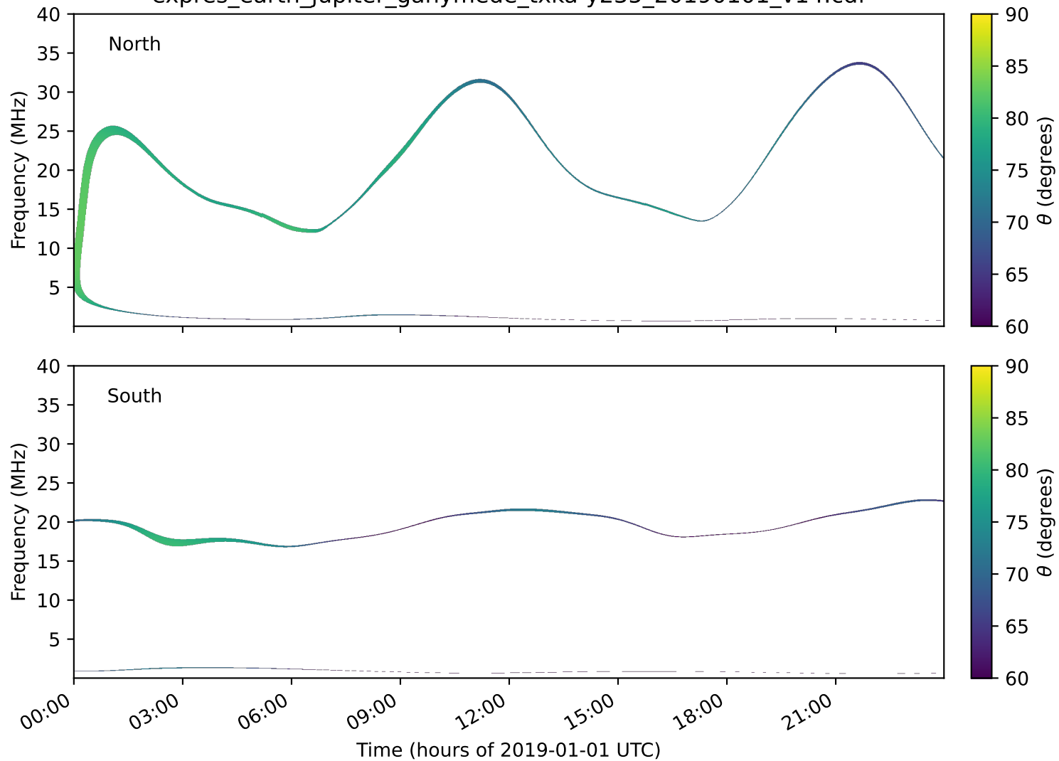
expres_earth_jupiter_ganymede_txka-y235_20190101_v14.cdf
