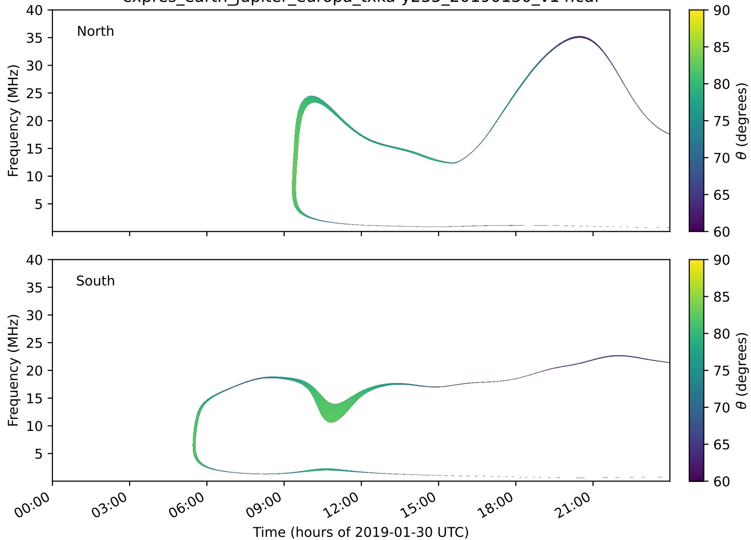
expres_earth_jupiter_europa_txka-y235_20190130_v14.cdf
