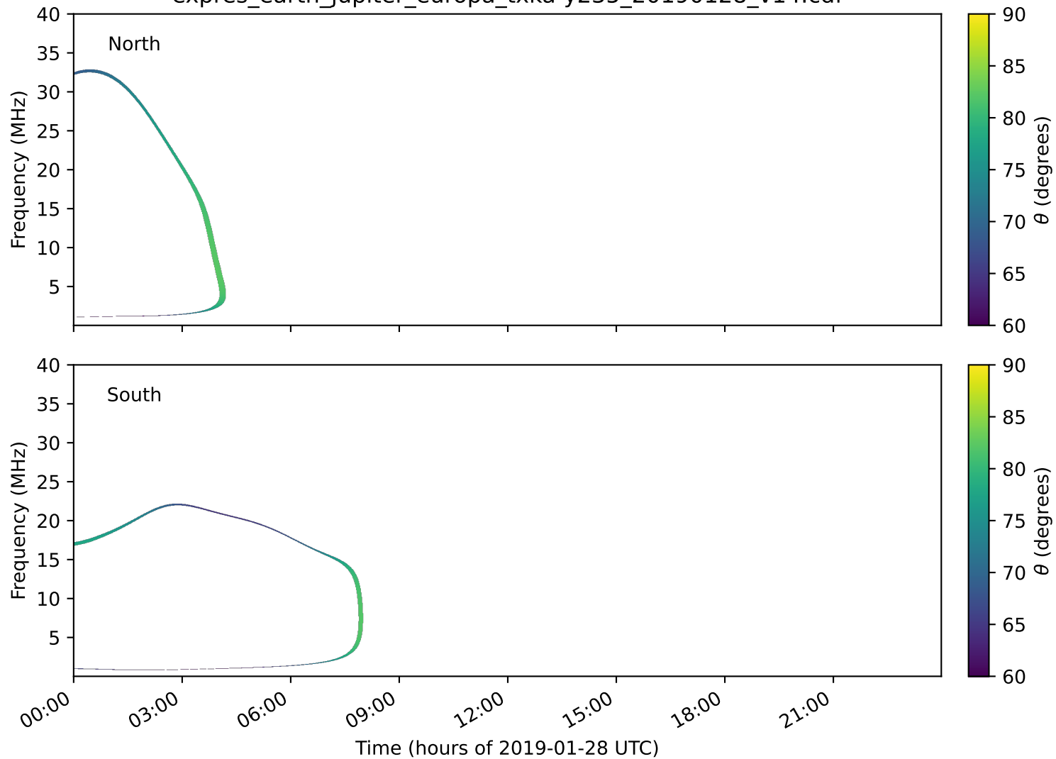
expres_earth_jupiter_europa_txka-y235_20190128_v14.cdf
