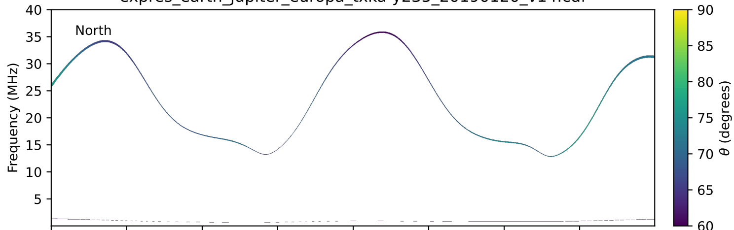
expres_earth_jupiter_europa_txka-y235_20190120_v14.cdf
