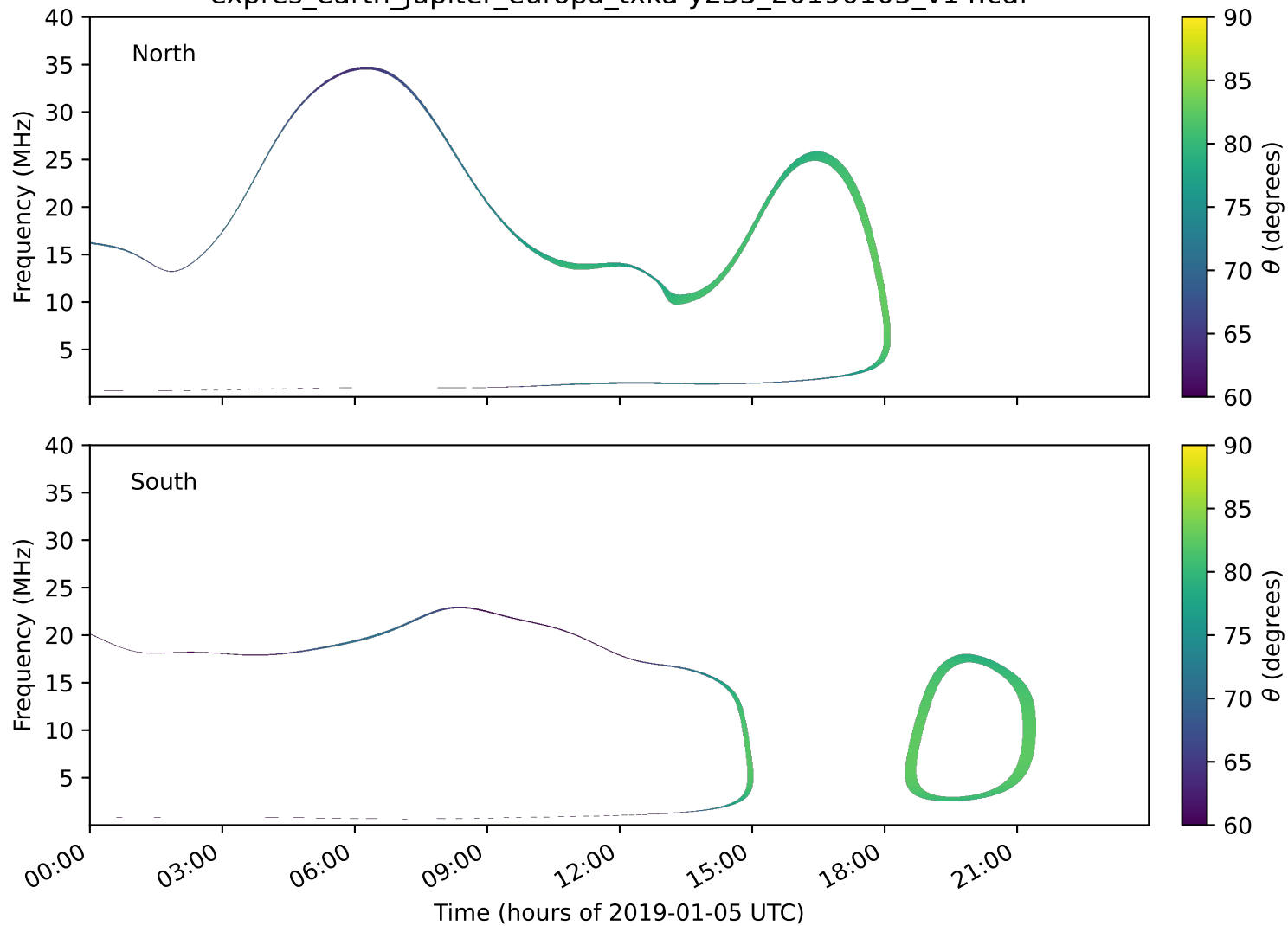
expres_earth_jupiter_europa_txka-y235_20190105_v14.cdf
