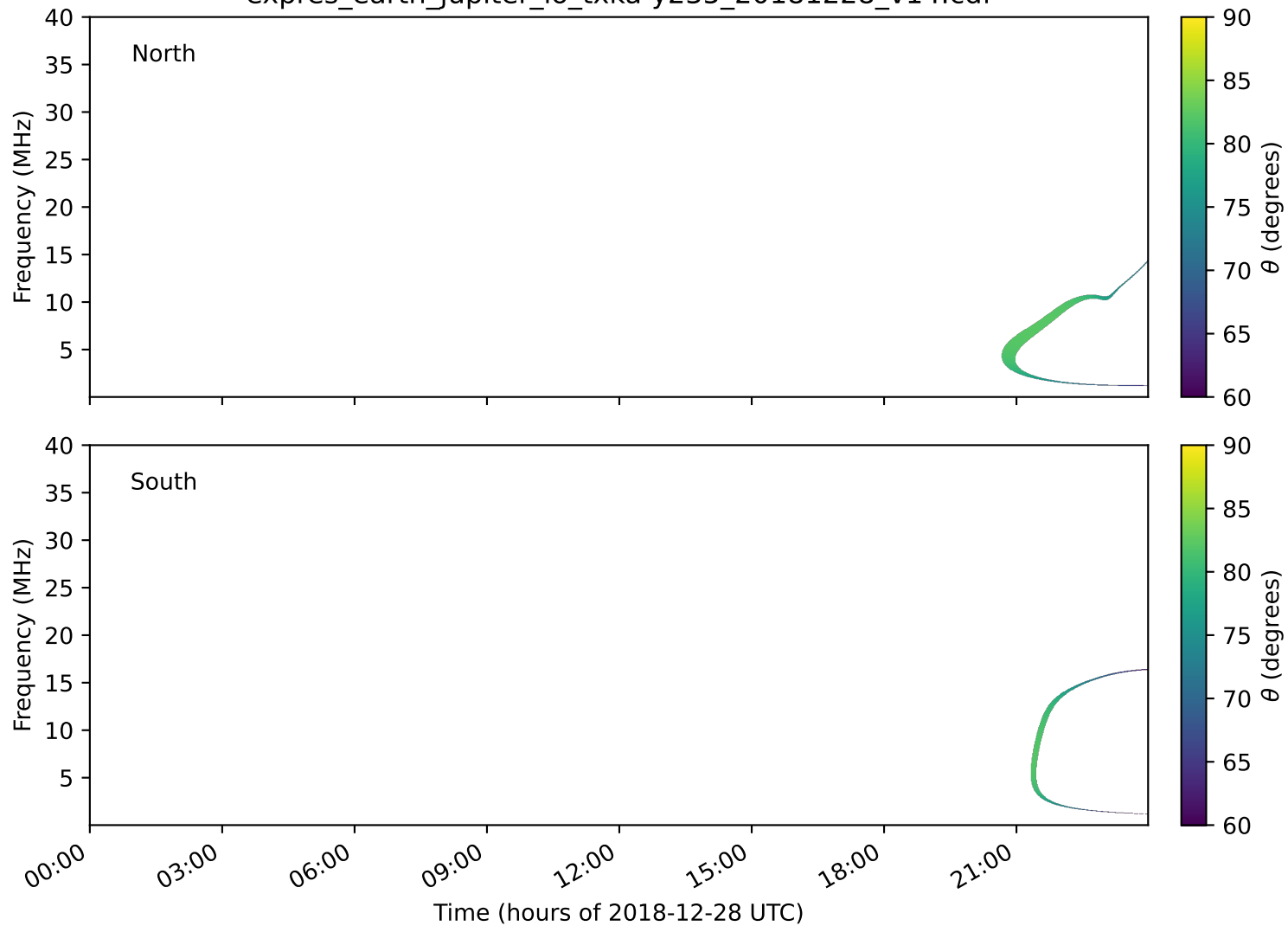
expres_earth_jupiter_io_txka-y235_20181228_v14.cdf
