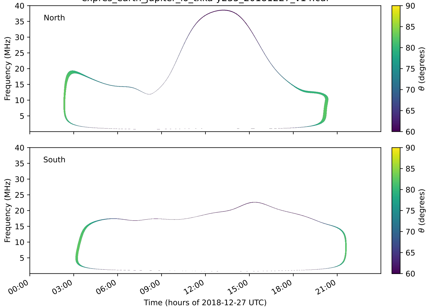
expres_earth_jupiter_io_txka-y235_20181227_v14.cdf
