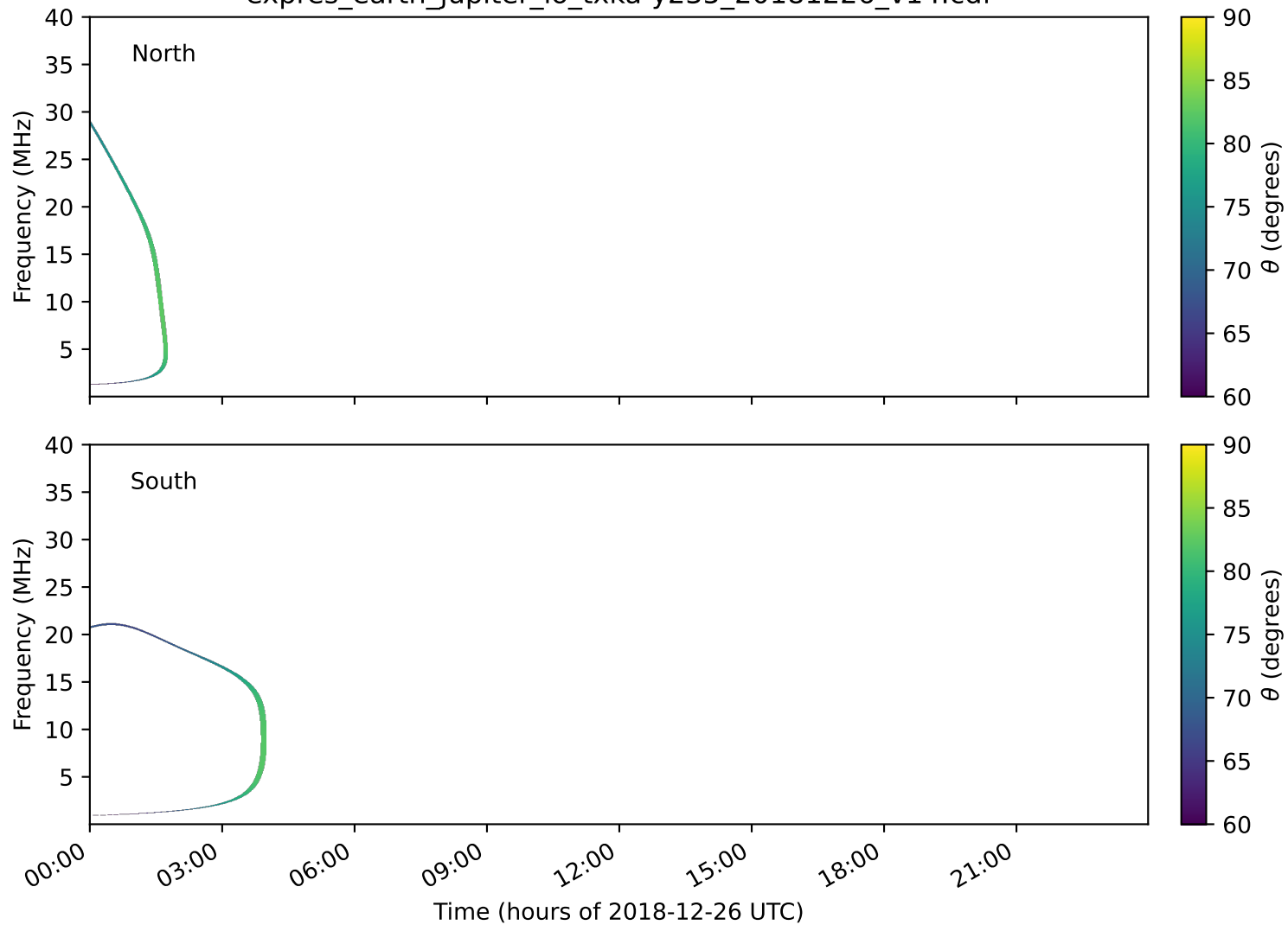
expres_earth_jupiter_io_txka-y235_20181226_v14.cdf
