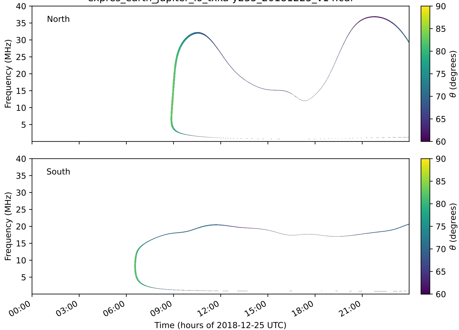
expres_earth_jupiter_io_txka-y235_20181225_v14.cdf
