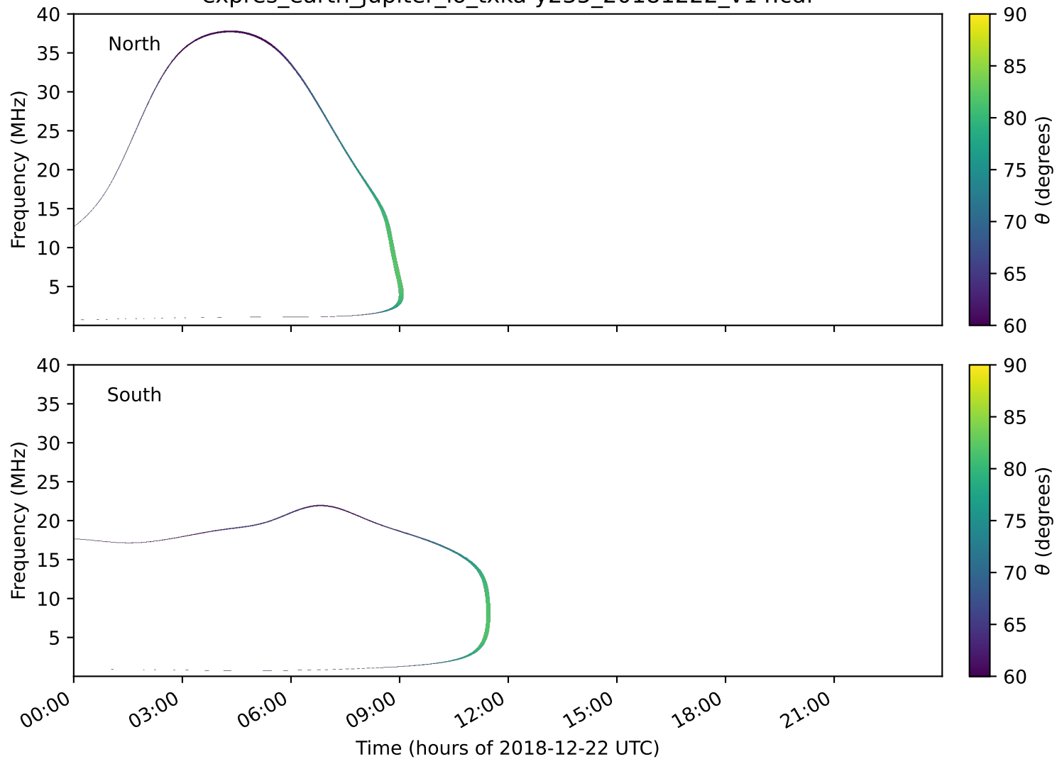
expres_earth_jupiter_io_txka-y235_20181222_v14.cdf
