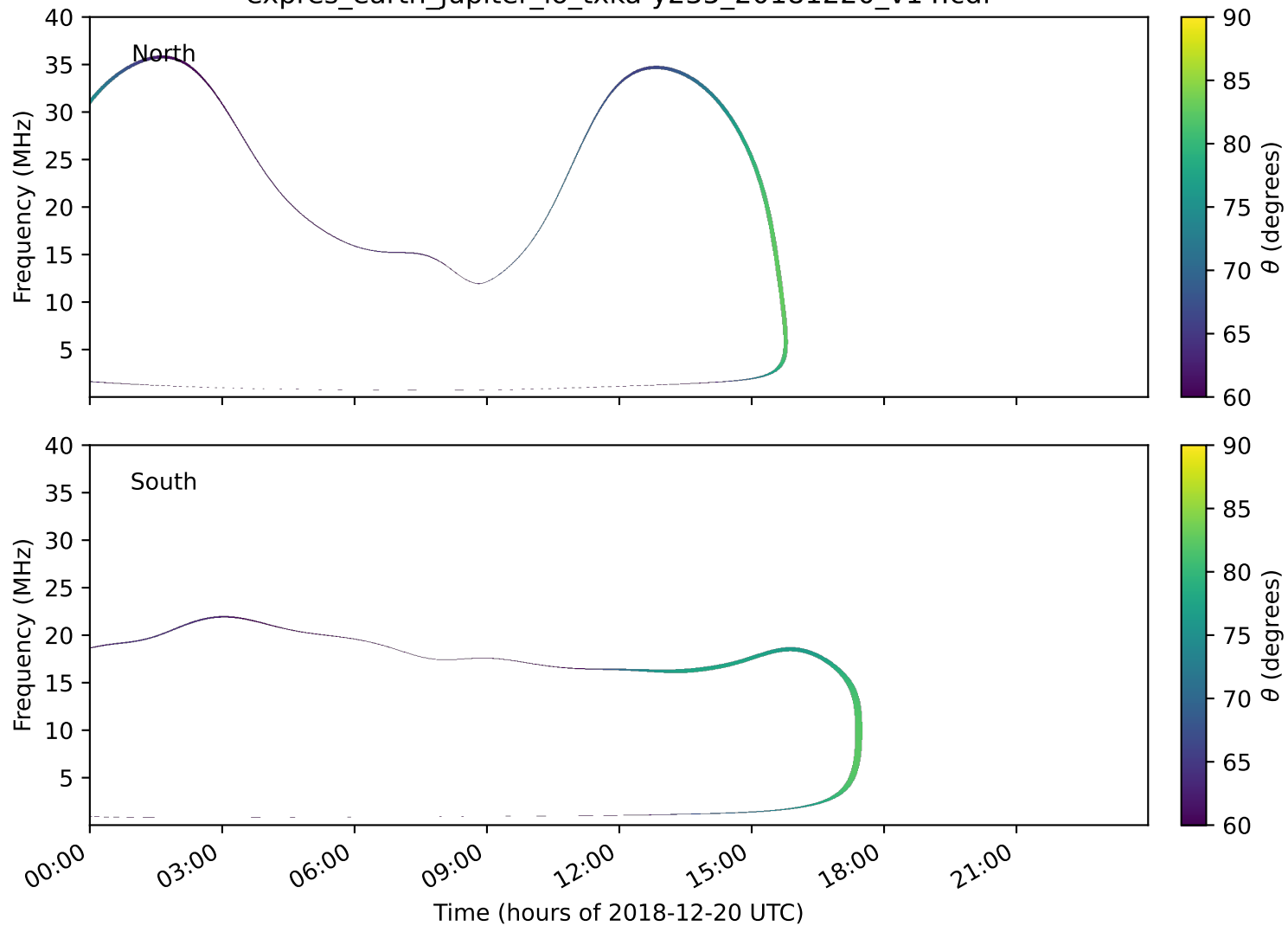
expres_earth_jupiter_io_txka-y235_20181220_v14.cdf
