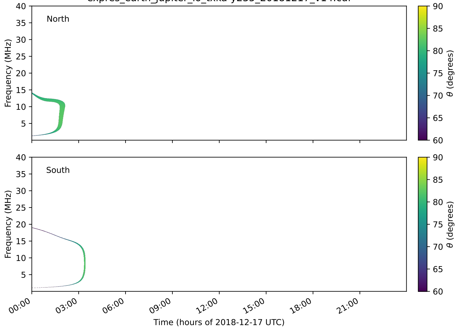
expres_earth_jupiter_io_txka-y235_20181217_v14.cdf
