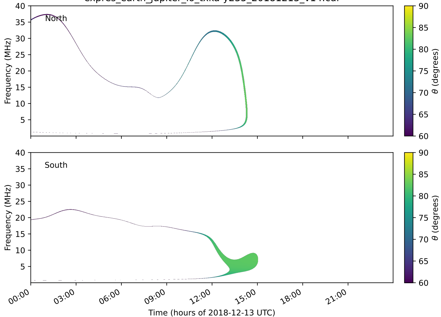
expres_earth_jupiter_io_txka-y235_20181213_v14.cdf
