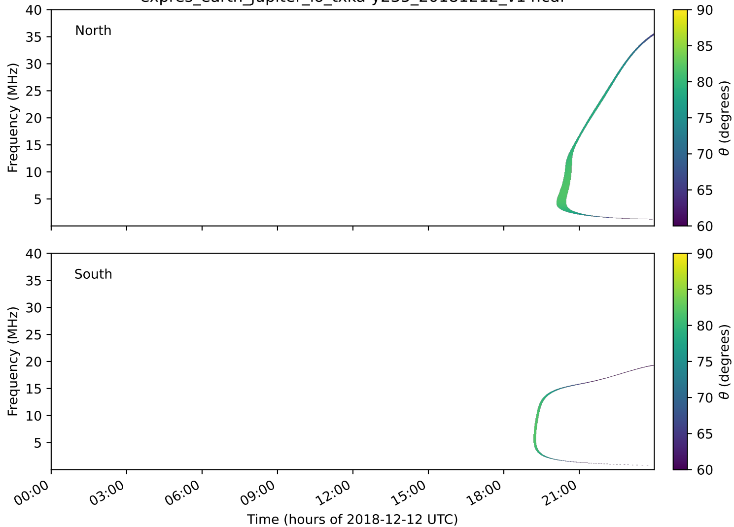
expres_earth_jupiter_io_txka-y235_20181212_v14.cdf
